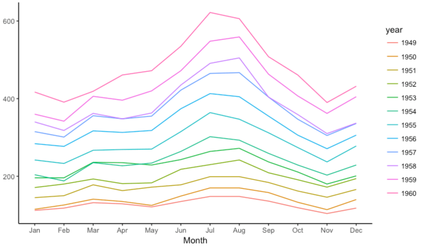
Seasonal plot: International Airline Passengers
